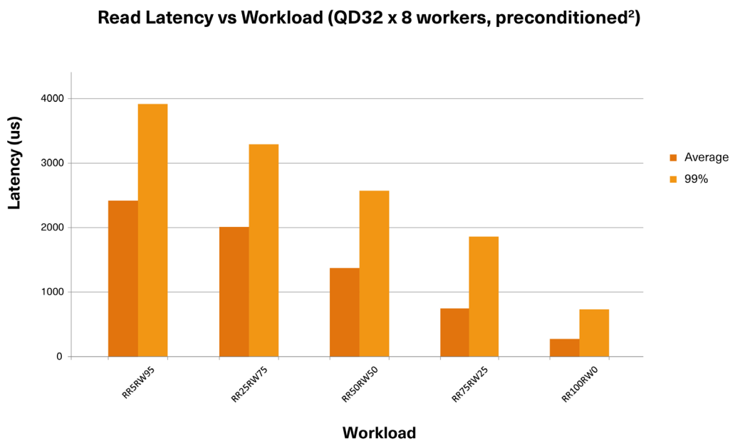
Figure 2: XD6 Series read latency on mixed workloads
