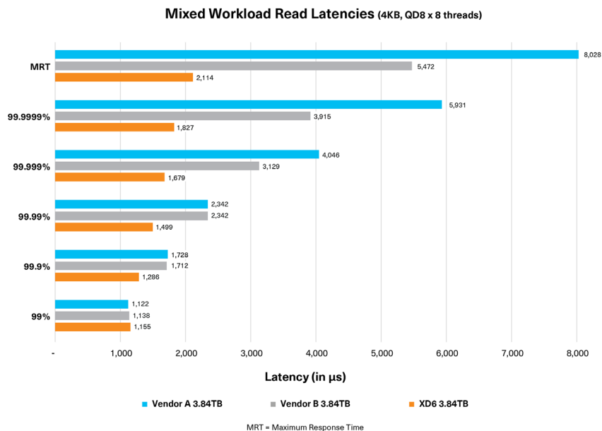
Figure 3: Mixed workload read latency QoS comparing the XD6 Series to two U.2 SSDs from leading vendors
